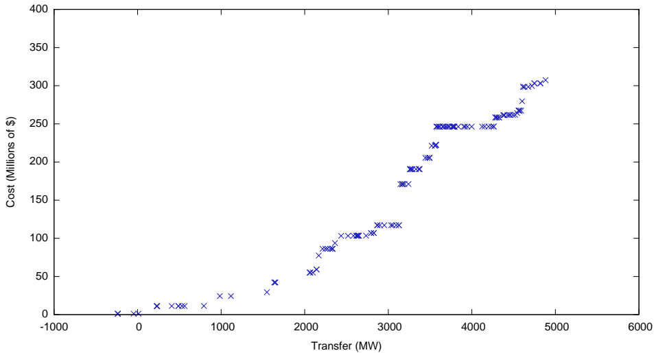
Transfer Capability vs. Cost Max Interface - All Sources - 2abg - Midwest ISO Sink
