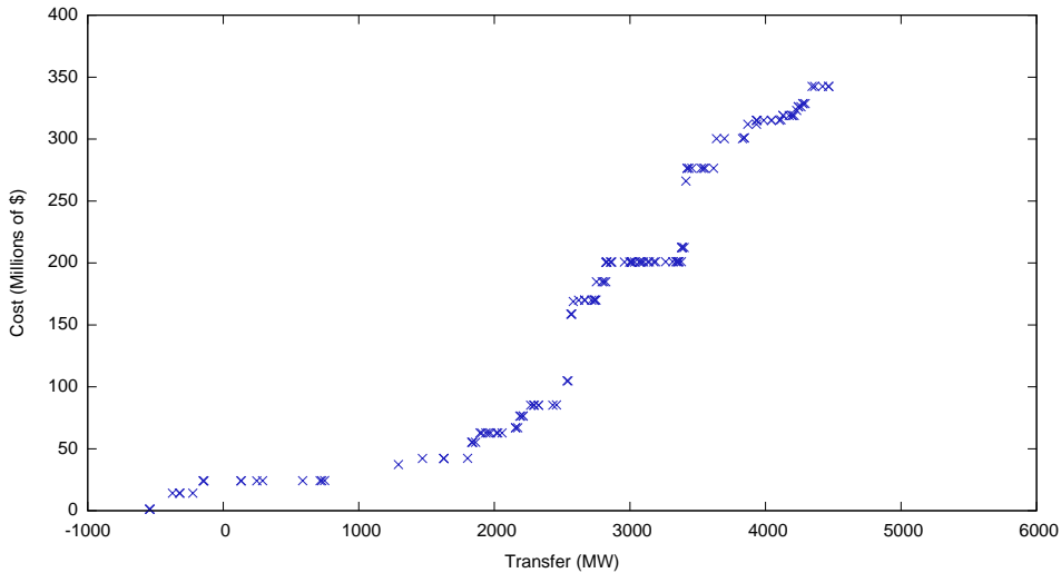
Transfer Cabability vs. Cost Max Interface - All Sources - 2abfg - Midwest ISO Sink
