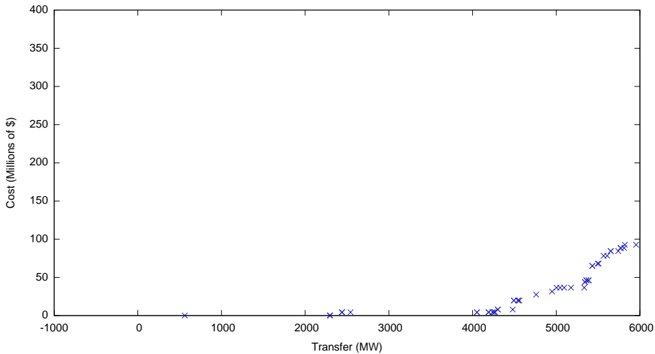
Transfer Cabability vs. Cost Historical Interface - All Sources - 2acd - Northern MAPP
