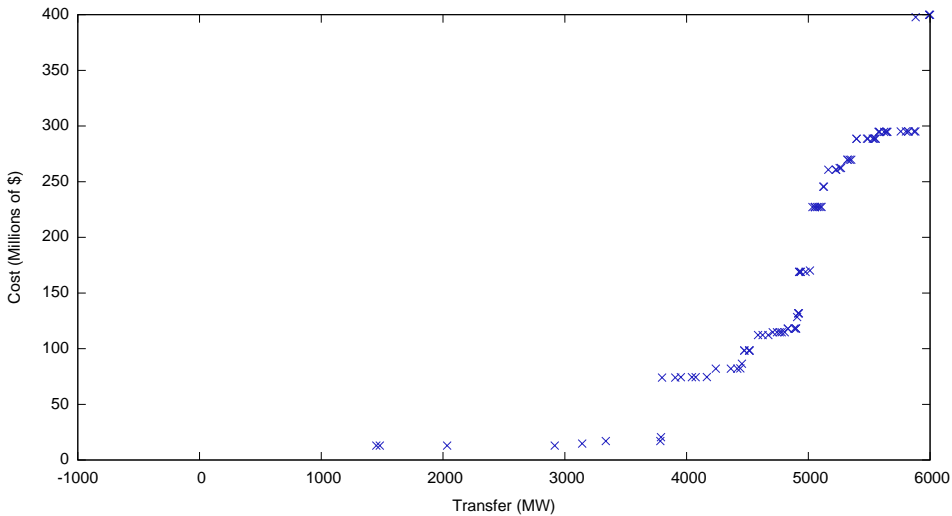
Transfer Cabability vs. Cost Historical Interface - All Sources - 2abd - Twin Cities Sink
